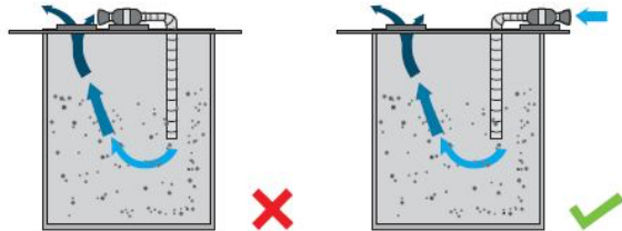
Force Ventilation
